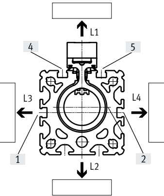
Piston Ø 32 ... 80
